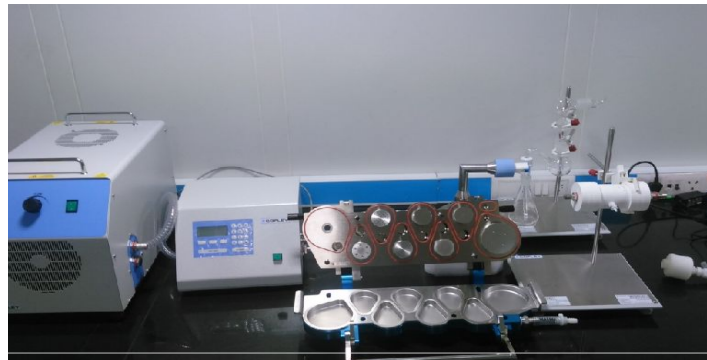
NGI for APSD (DPI /MDI) Testing
